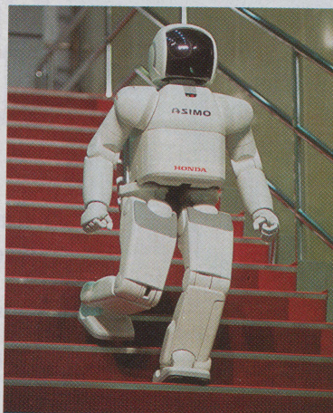
ALL UNDER CONTROL — Honda’s robot Asimo can climb or descend stairs, kick a ball, and shake hands, but requires an energy-intensive motor for each of 26 joints.
