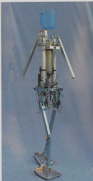
LADYLIKE LOCOMOTION — Denise, a robot built at Delft University, takes a graceful and energy-efficient step by relying on natural dynamics.
