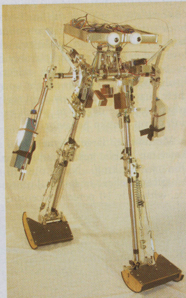
STEPPING UP — This energy-efficient robot from Cornell University has inspired new prosthetic designs.
